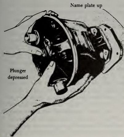
FIGURE 4-47. Installing a magneto.
